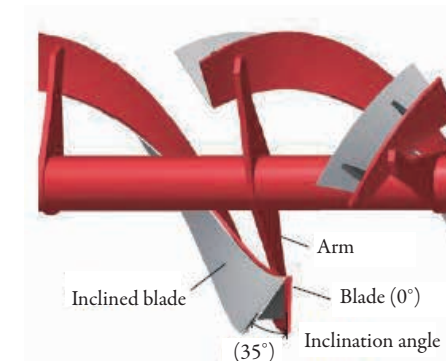
Figure 1: Blade inclination angle
