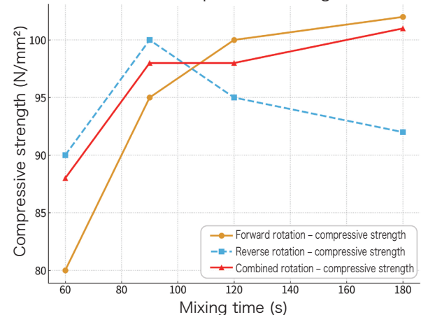
Relationship between mixing time and compressive strength
