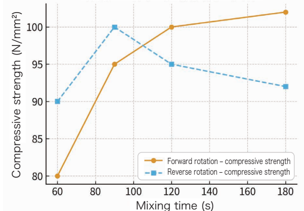
Figure 7: Relationship between mixing time and compressive strength
