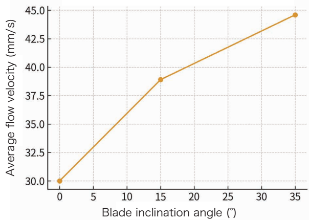
Figure 5: Relationship between blade inclination angle and average flow velocity
