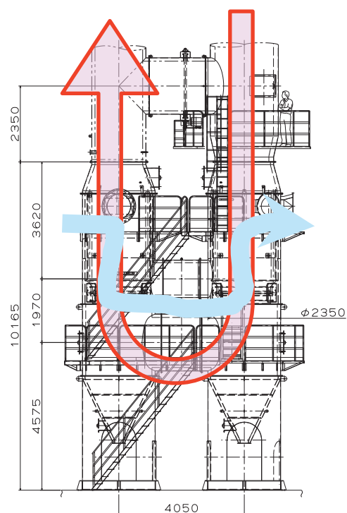
Fig7 Side view of the heat exchanger
