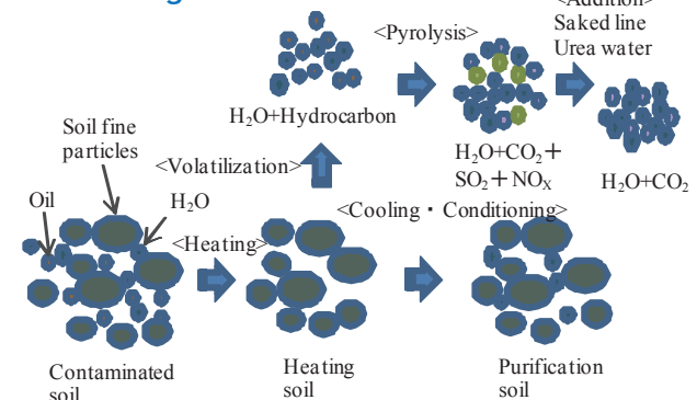
Fig1 Conception diagram of the purification by the heating
